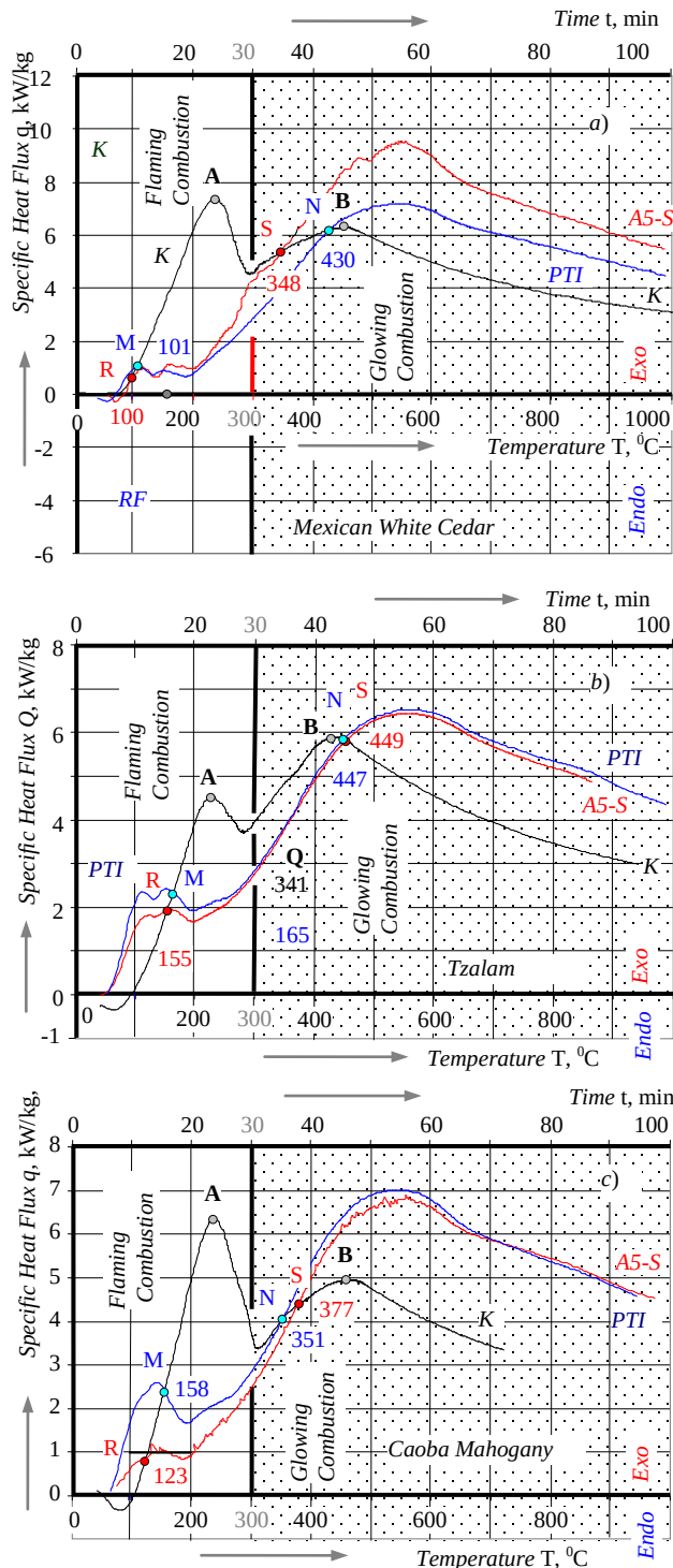
Fig. 4. Criterion of wood pyrolysis and combustion behavior established on simultaneous thermal analysis (STA) - specific heat flux q spectra (per unit surface and mass losses) of bare wood sample (K), plasma-aided flame retarded sample (PTI) and plasma-aided flame retarded sample with FR-solution modified by anionic (5 vol. %) and siloxane surfactant or super spreader (0.1 %) (A5-S): a - Mexican White Cedar ( Cupressus Lusitanica ); b - Tzalam ( Lysiloma bahamensis ); c - Mahogany Caoba ( Swietenia macrophylla ).
