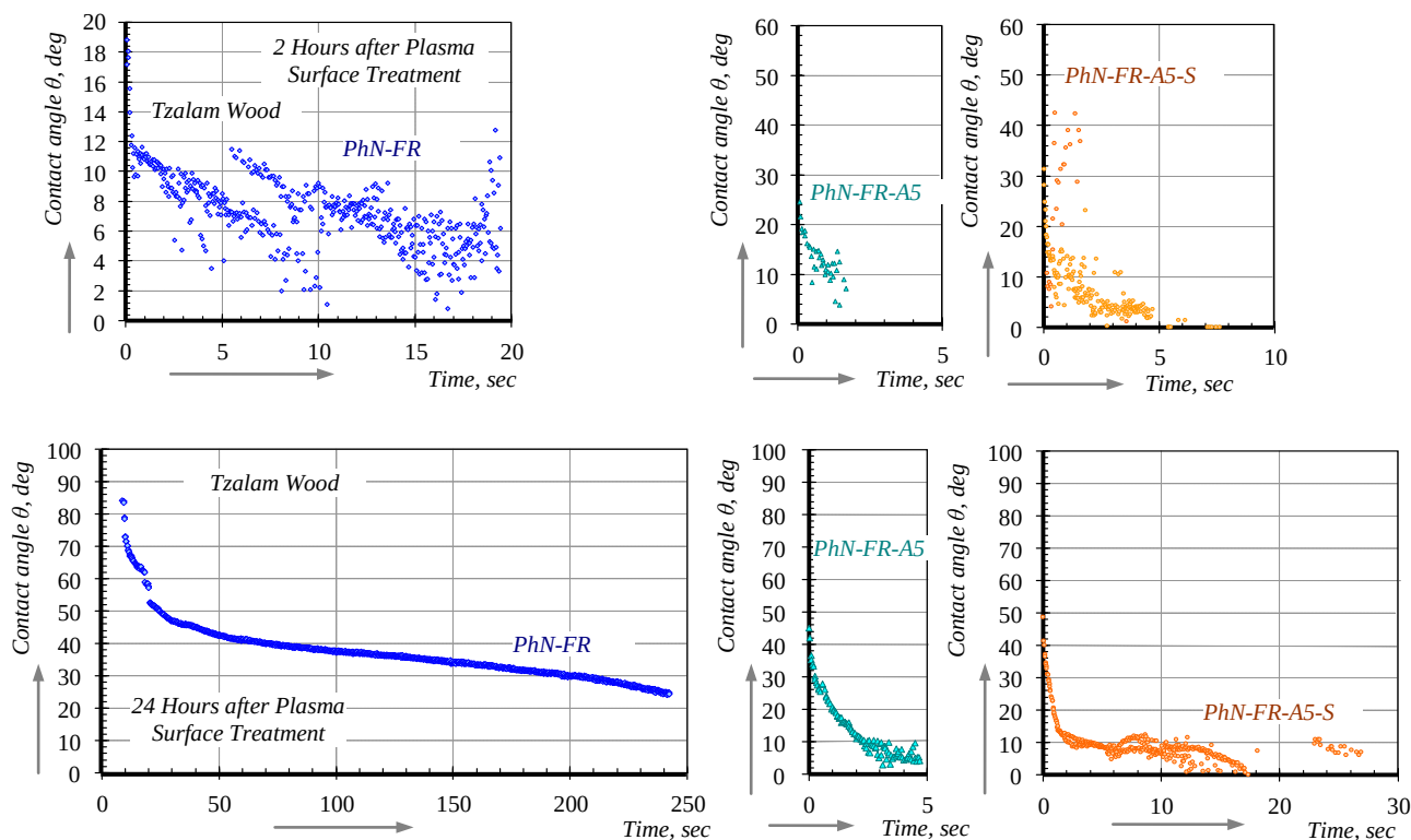
Fig. 3. Time-depending change of contact angle \theta of a FR-water solution as it advances slowly over a non-ideal (wood) surface (e.g., not chemically homogeneous, rough or not perfectly smooth, and porous as in the case of most practical wood surfaces): PhN-FR - 30 mass % water impregnation solution of phosphor and nitrogen containing flame retardant; PhN-FR-A5 - water solution with 5 vol. % anionic surfactant; PhN-FR-A5-S - water solution with 5 vol. % anionic surfactant and 0.1 vol. % spreader; PhN-FR-A10-S - water solution with 10 vol. % anionic surfactant and 0.1 vol. % spreader - 2 (a) and 24 (b) hours old surfaces - after atmospheric dielectric barrier discharge (DBD) surface treatment in air.
