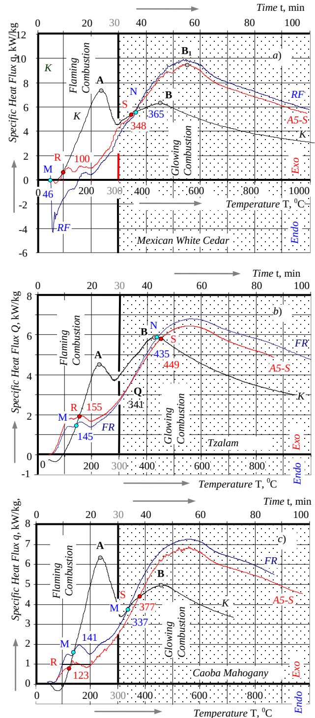
Fig. 5. Criterion of wood pyrolysis and combustion behavior established on simultaneous thermal analysis (STA) - specific heat flux q spectra (per unit mass losses) of bare wood sample (K), flame retarded sample (FR), and plasma-aided flame retarded sample with FR-solution modified with anionic (5 vol. %) and siloxane surfactant (0.1 %) (A5-S): a - Mexican White Cedar ( Cupressus Lusitanica ); b - Tzalam ( Lysiloma bahamensis ); c - Mahogany Caoba ( Swietenia macrophylla ).
