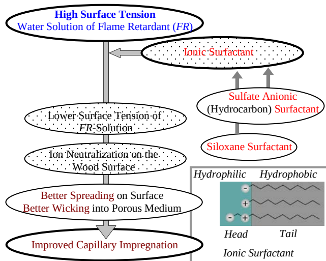
Fig. 1. The main objectives of plasma-aided capillary impregnation technology (PACI) are both increasing of wood surface energy by plasma-chemical surface pre-treatment and decreasing of surface tension of impregnating FR-solution by ionic non-organic and siloxane surfactants ( surface-active agents ).
